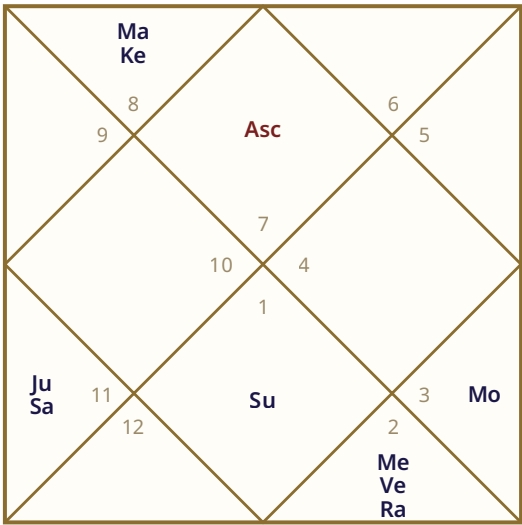
Navamsa (D9)
